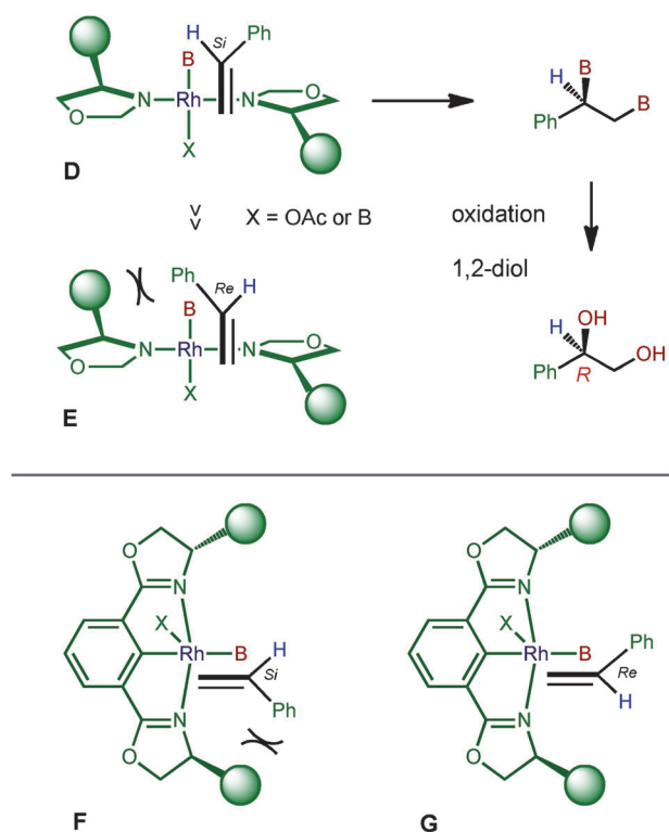
Figure 3. Proposed transition state. Boryl group at apical position and syn diboration to Si face of the \alpha -carbon atom (D and E). The equatorial boryl structures F and G.
